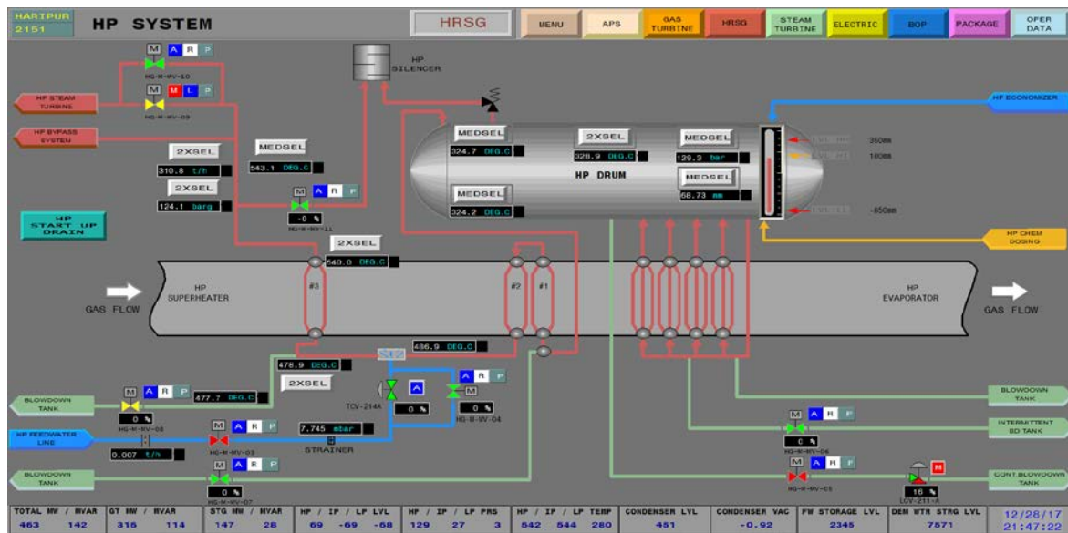
Components in a DCS screen
